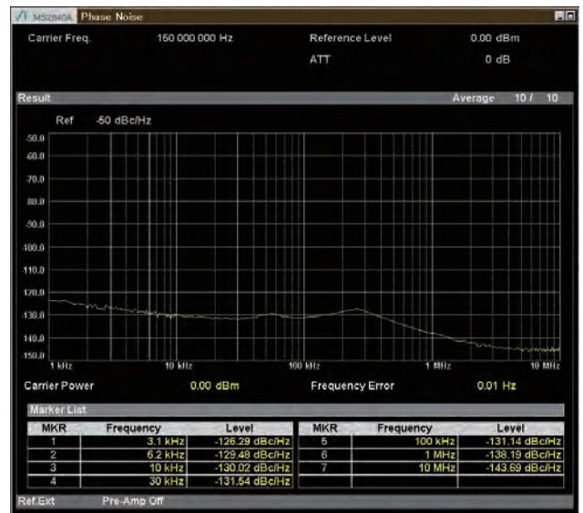
Phase Noise Measurement 150 MHz Measurement Frequency, Preamp Off
